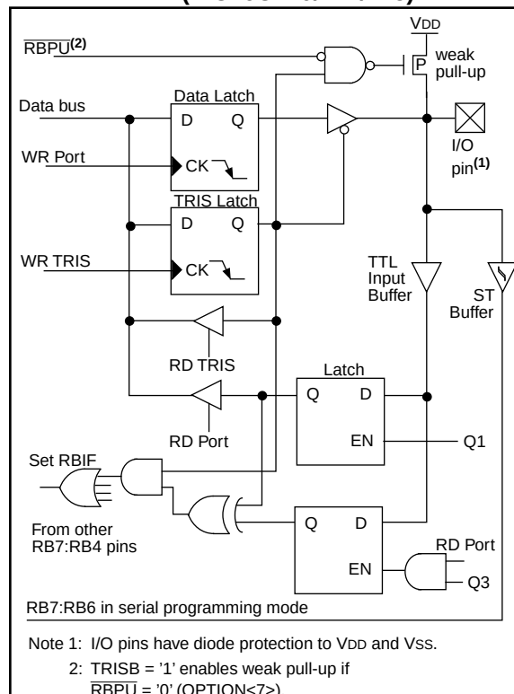
FIGURE 5-5: BLOCK DIAGRAM OF RB7:RB4 PINS (PIC16C710/711/715)
