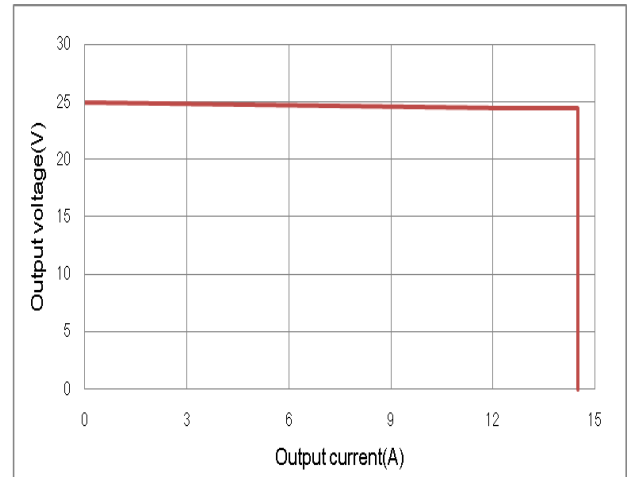
Figure 4: Output voltage vs. Output current OCL Performance @72Vin
