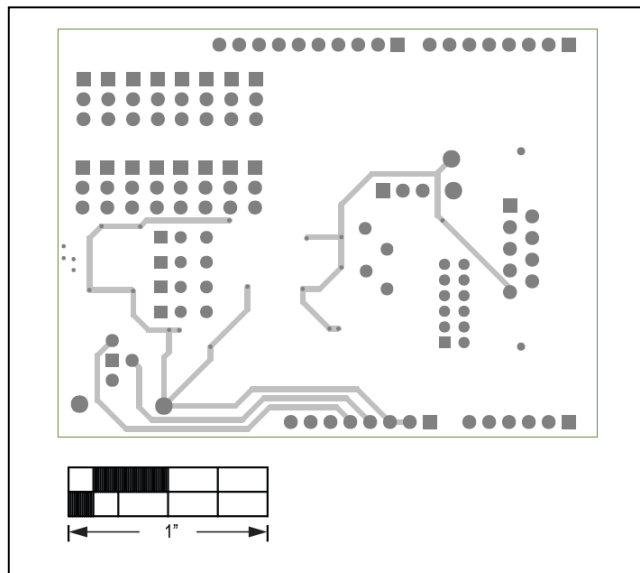
MAX33250E Shield—Internal 2
