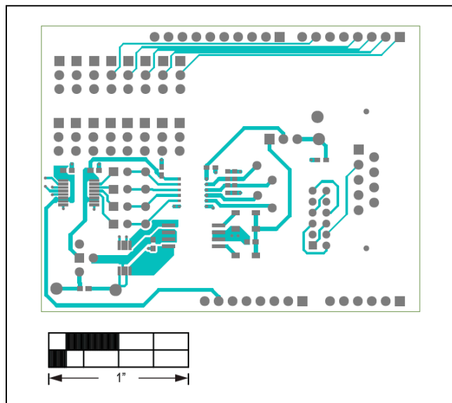
MAX33250E Shield—Top
