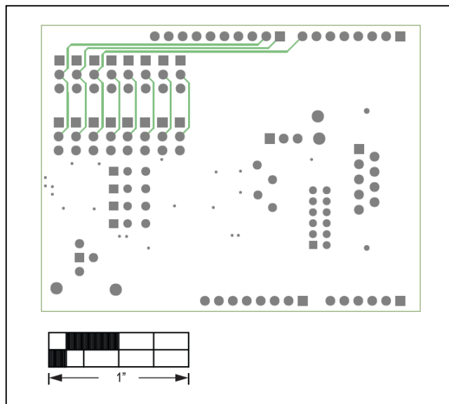
MAX33250E Shield—Internal 3
