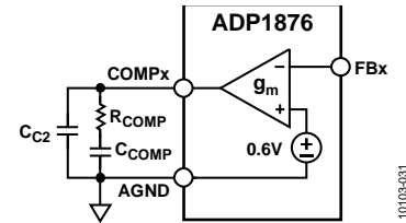
Figure 31. Compensation Components
