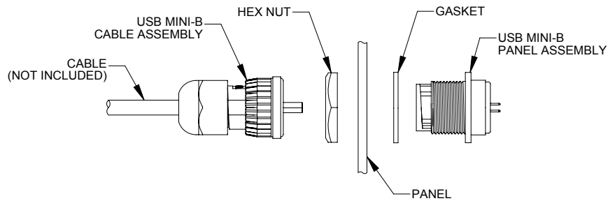
DCC-USBNB-160 USB Mini-B Cable Plug Field Installable
