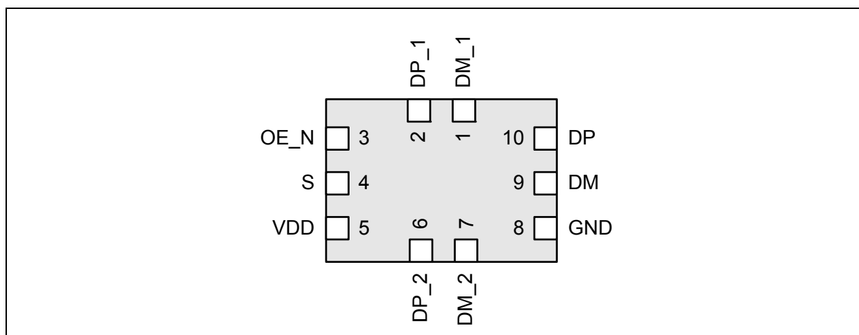
Figure 2.1 USB3740 Package Diagram
