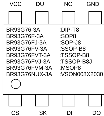
Figure 3. Pin Configuration
