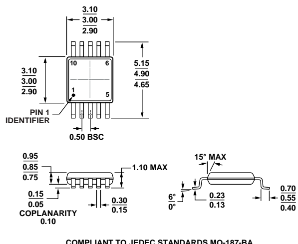
Figure 49. 10-Lead Mini Small Outline Package [MSOP] (RM-10)
