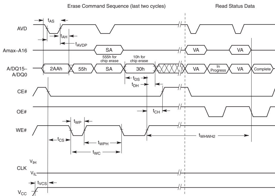
Erase Command Sequence (last two cycles)
