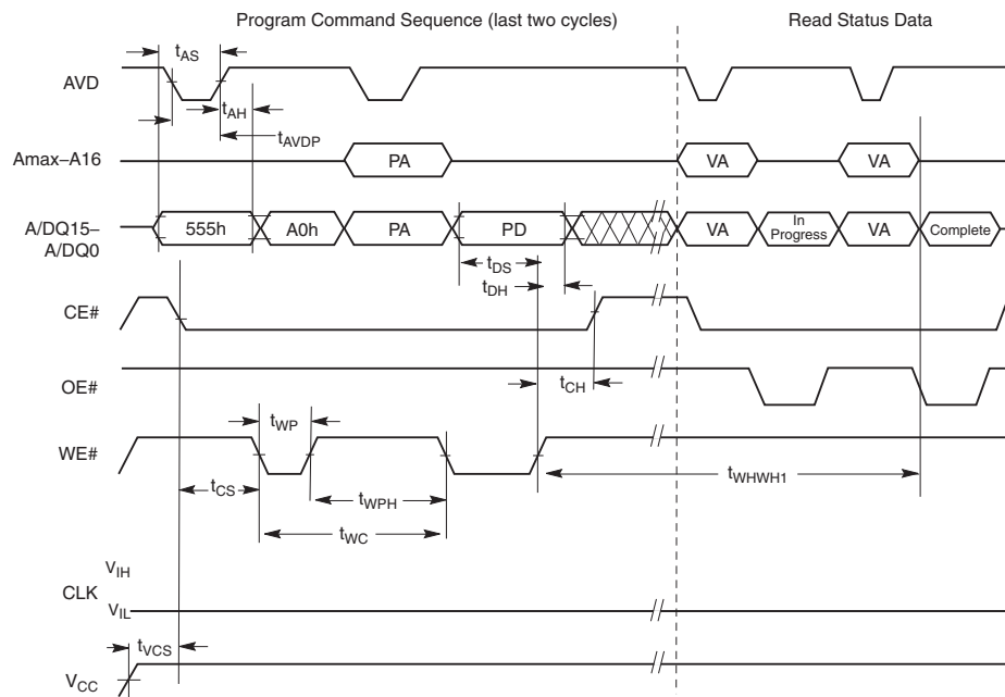
Program Command Sequence (last two cycles)
