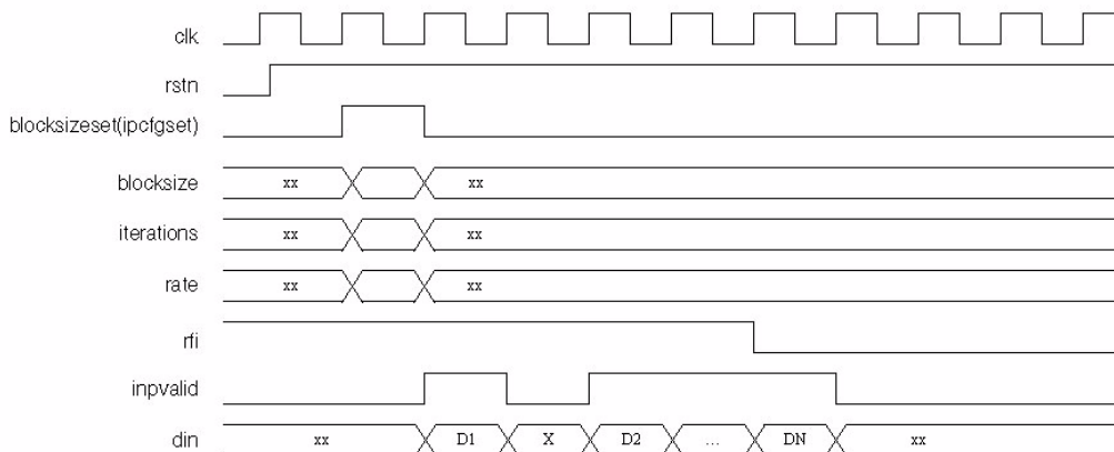
Figure 6. Input Data Handshaking with ininvalid Going Low
