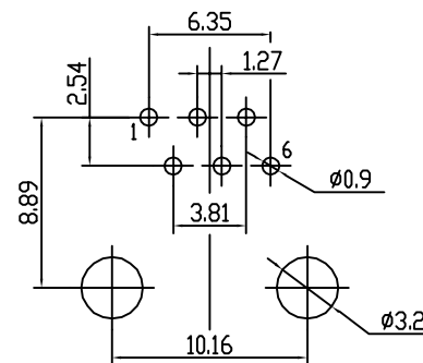
6P6C
