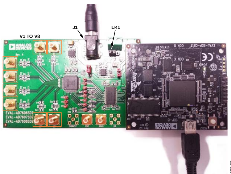
Figure 1. Evaluation Board (Left) Connected to the SDP Board (Right)
