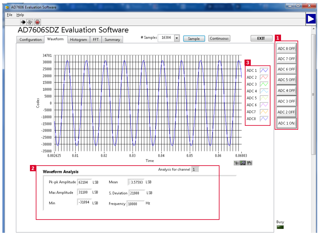
Figure 13. Waveform Tab
