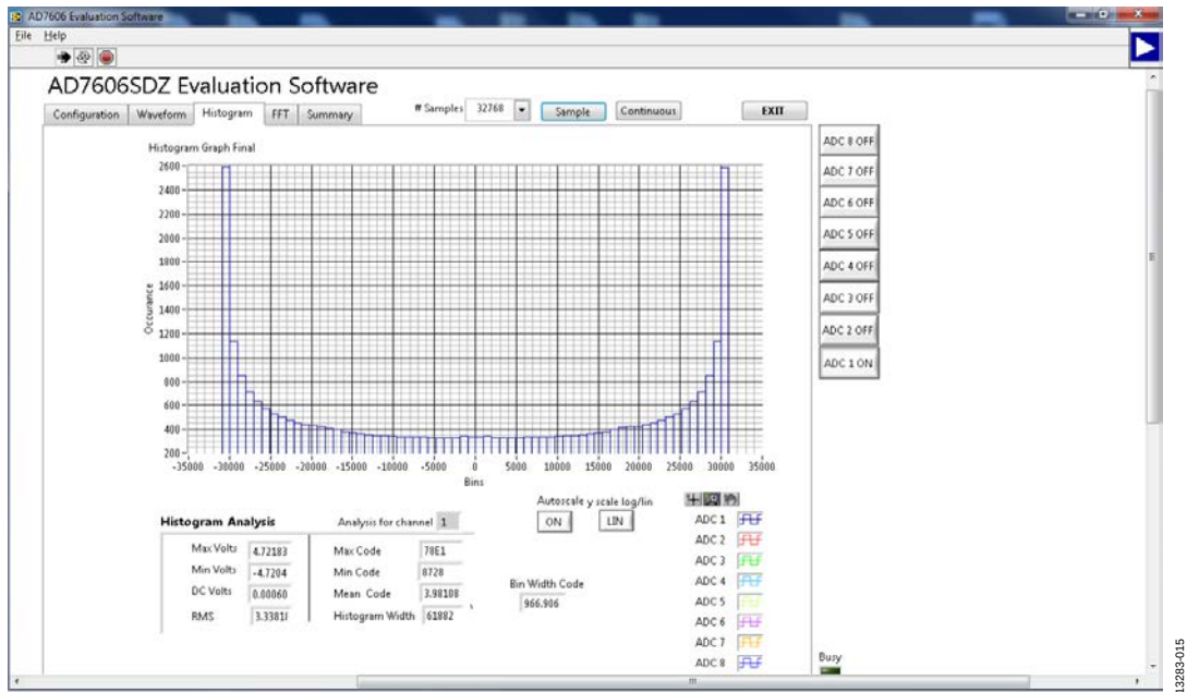
Figure 14. Histogram Tab
