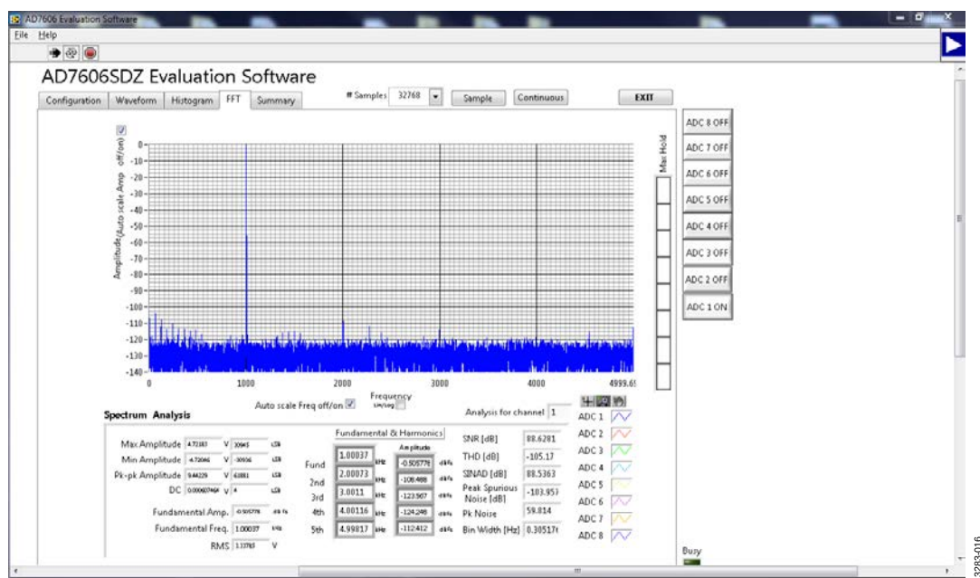
Figure 15. FFT Tab
