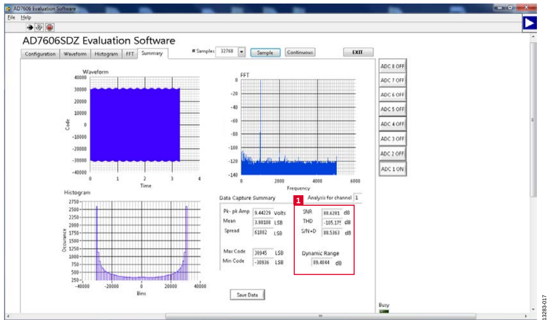
Figure 16. Summary Tab
