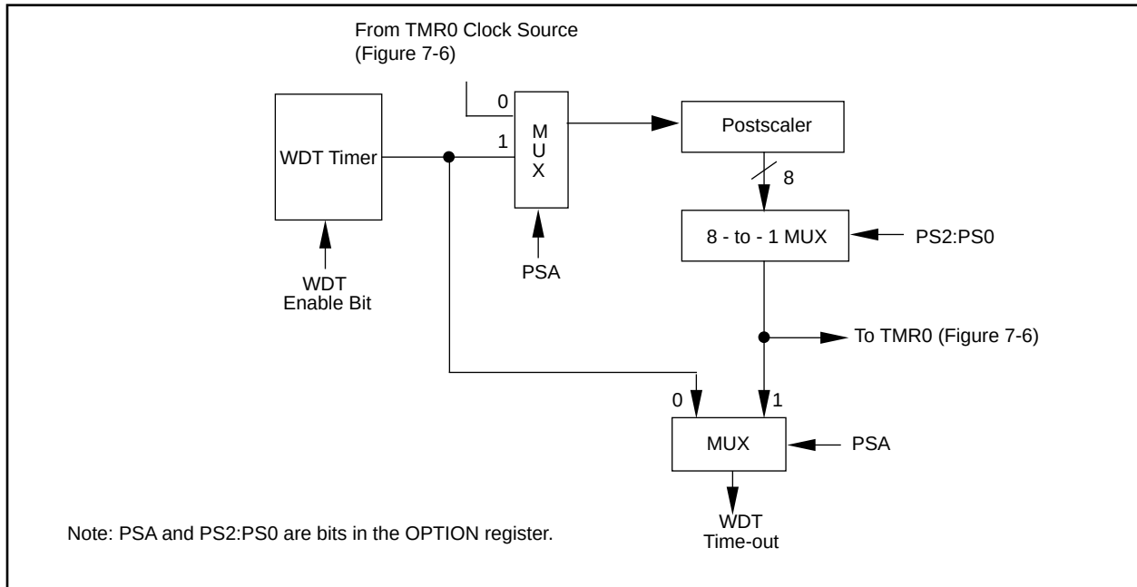
FIGURE 9-17: WATCHDOG TIMER BLOCK DIAGRAM
