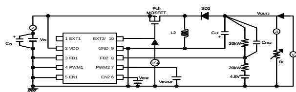
Circuit 6
