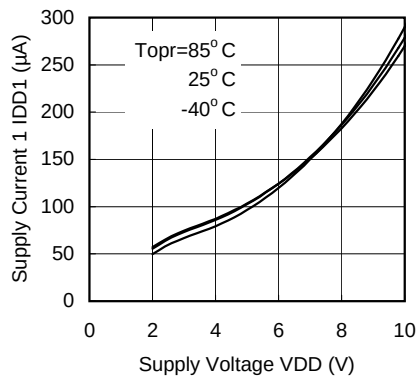
(11) Supply Current 1-2 vs. Supply Voltage
