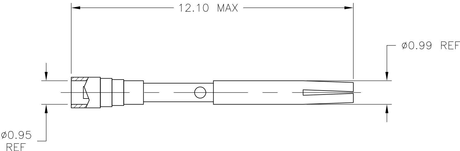
CENTER CONTACT
