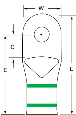
MC1-14RX
