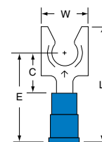
MV14-14FL
