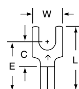
MU18-8FB 8 22-18
