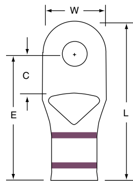
MC2-14RX
