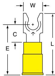
MVU10-10FL
