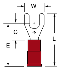
MNG18-8F
