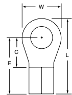
MU4-38RHT Stud Size 3/8 Wire Range 4
