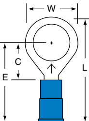
MVU14-38R
