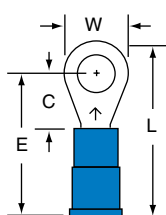
MVU14-10R
