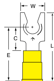
MVU10-14FL
