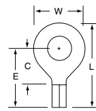
MU14-14RHT Stud Size 1/4 Wire Range 16-14
