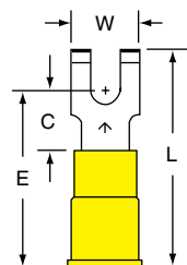
MVU10-6FFBK
