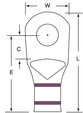
MC2-38RX
