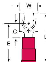
MV18-10FL
