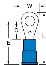
MV14-8R/L
