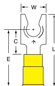
MV10-14FL
