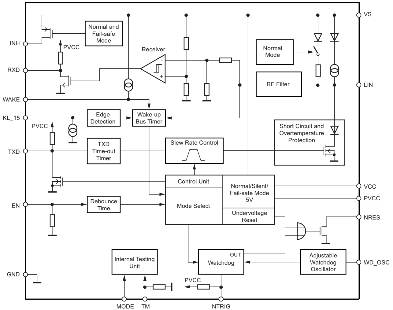
Figure 3-1. Block Diagram
