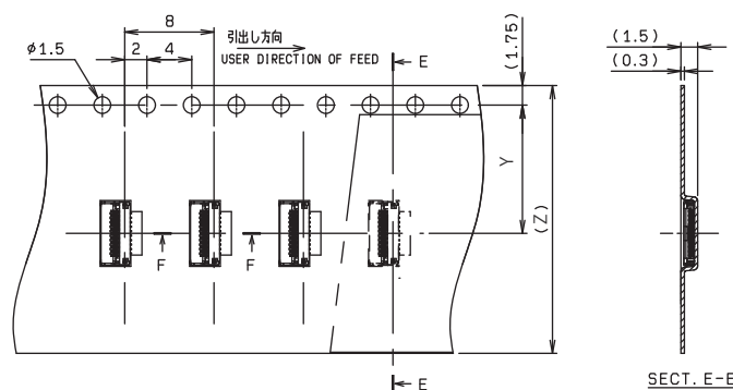
REEL DIMENSION
