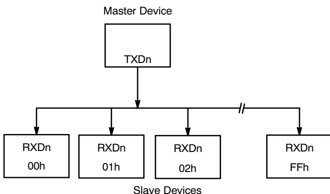
Figure 51. An Illustration Depicting the Concept of Multi-Drop Mode
