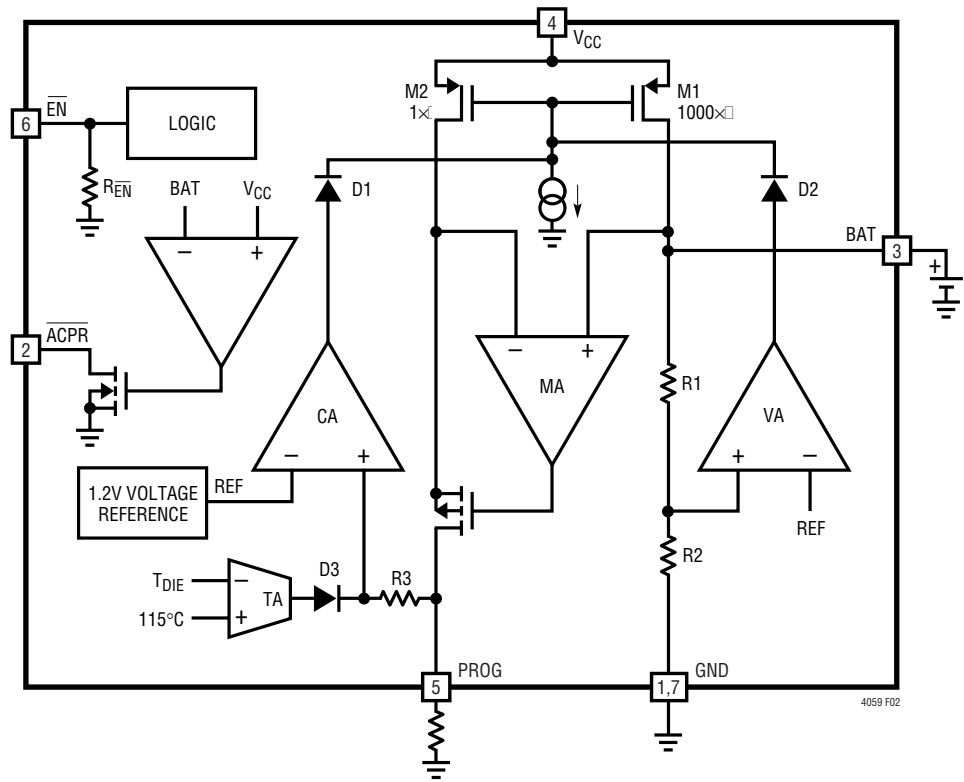
Figure 2 (LTC4059A)
