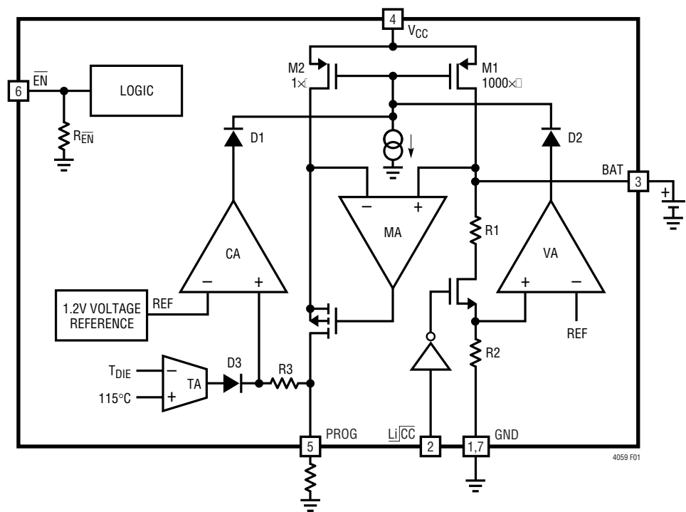
Figure 1 (LTC4059)
