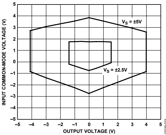
Figure 10. Input Common-Mode Voltage vs. Output Voltage, V_S = \pm 2.5\text{ V}, \pm 5\text{ V}; G = 10
