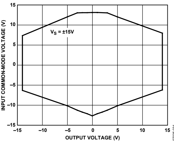
Figure 11. Input Common-Mode Voltage vs. Output Voltage, V_S = \pm 15\text{ V}, G = 10
