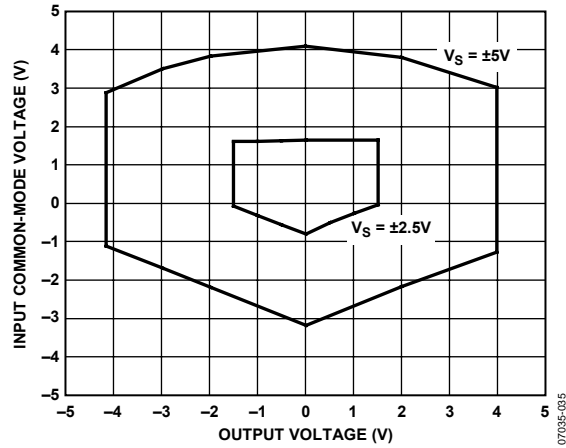
Figure 12. Input Common-Mode Voltage vs. Output Voltage, V_S = \pm 2.5\text{ V}, \pm 5\text{ V}; G = 100
