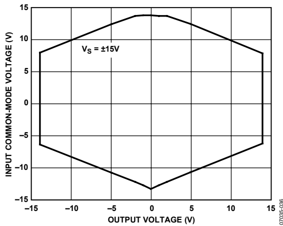
Figure 13. Input Common-Mode Voltage vs. Output Voltage, V_S = \pm 15\text{ V}, G = 100
