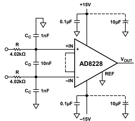
Figure 47. RFI Suppression
