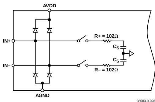
Figure 28. Simplified Analog Input
