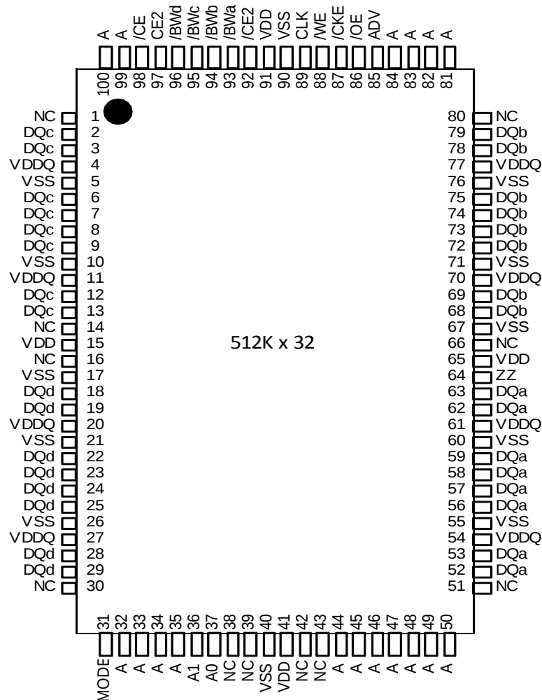
512K x 32, 100PIN QFP (Top View)
