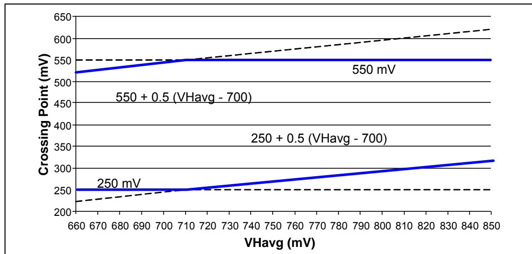
Figure 33-10. Differential Clock Cross Point Specification
