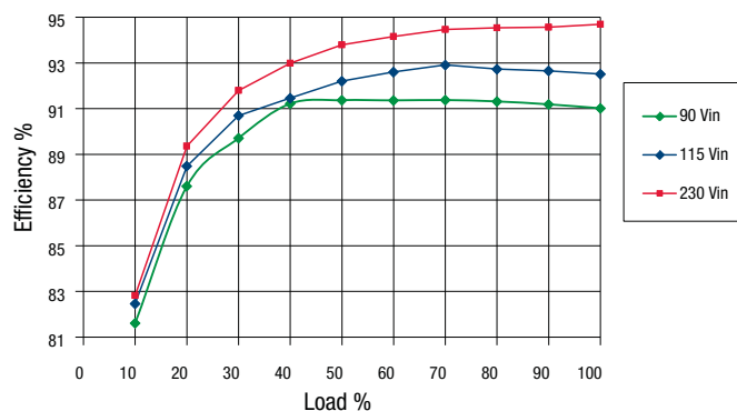
MVAC250-24F Efficiency
