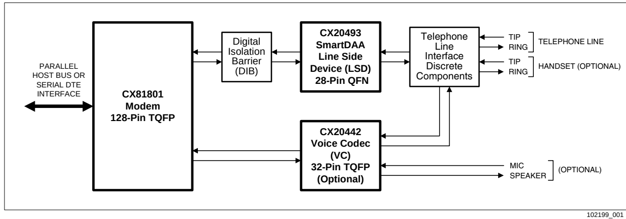
Figure 1-2. SmartV.XX Modem Major Interfaces
