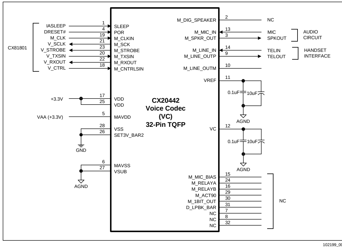
Figure 3-8. CX20442 VC 32-Pin TQFP Pin Signals
