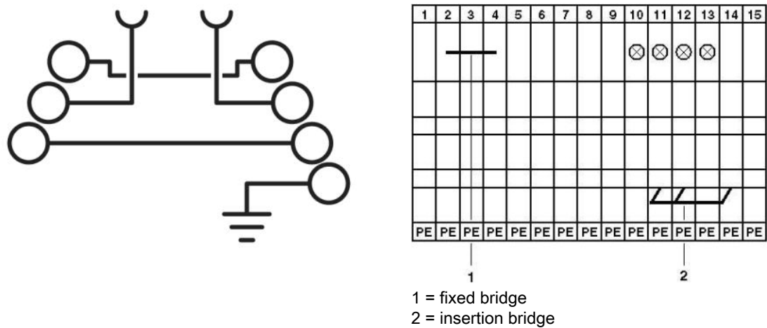
Circuit diagram
