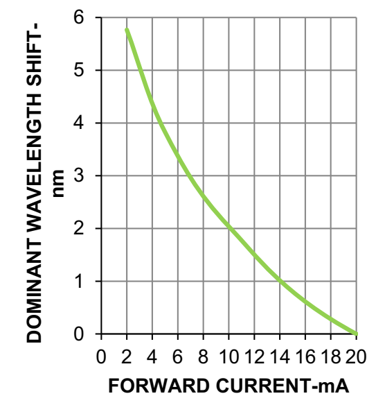
Figure 6: Wavelength Shift vs. Forward Current
