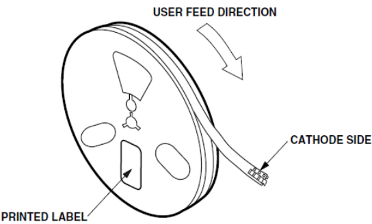
Figure 12: Reel Orientation
