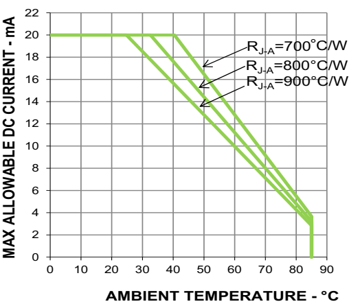
Figure 10: Derating Curve
