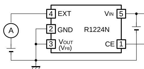
EXT “L” Output Current
