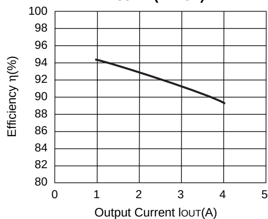
R1224N332M ( V_{IN}=5V )
