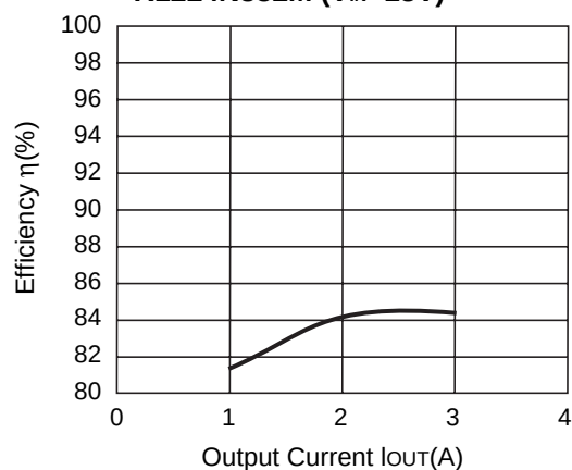
R1224N332M ( V_{IN}=18V )
