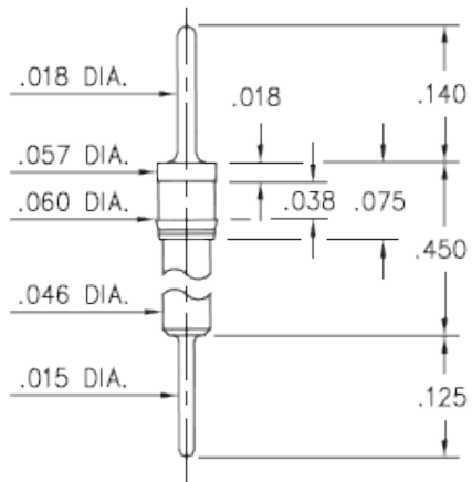
8885-0-00-XX-00-00-03-0 Press-fit in .057 mounting hole
