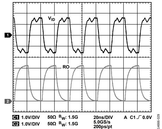
Figure 32. Receiver Propagation Delay (Oscilloscope Plot) at 50 Mbps, |V_{IO}| \geq 1.5 V
