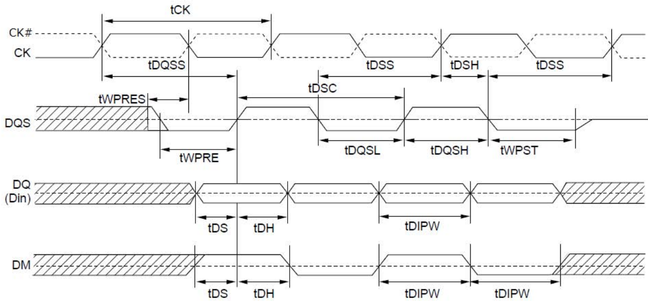
Figure 5.3 Write Timing Definition
