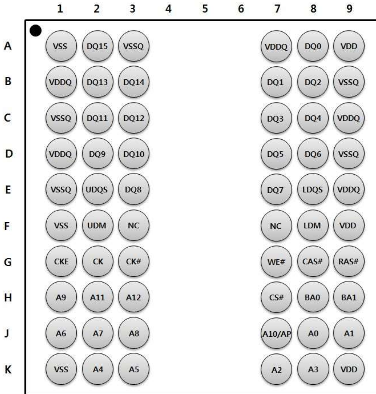
Figure 2.2 Pin configurations
