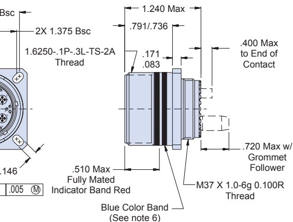
00-Wall Mount Receptacle With Slotted Holes
