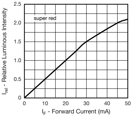
Fig. 6 - Relative Luminous Intensity vs. Forward Current (super red)
