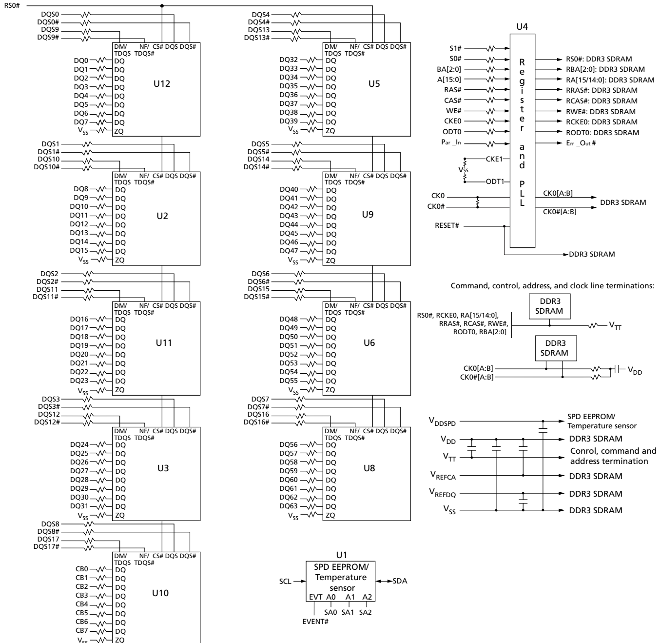
Figure 4: Functional Block Diagram RC A1 (PCB 1486)
