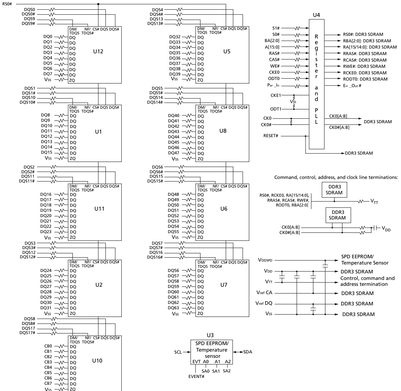
Figure 3: Functional Block Diagram R/C A (PCB 0692)
