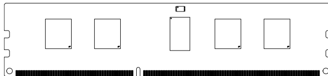
Figure 2: 240-Pin RDIMM (MO-269 R/C A1 – PCB 1486)
