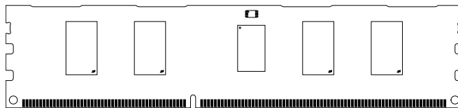
Figure 2: 240-Pin RDIMM (MO-269 R/C A1 – PCB 1486)
