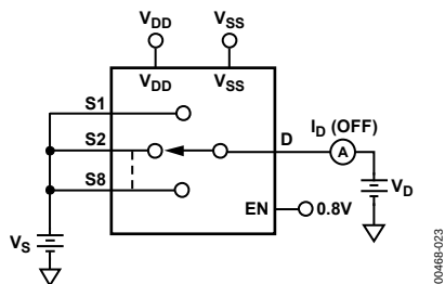
Figure 19. I_D (Off)
