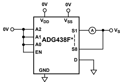
Figure 22. Input Leakage Current (with Power Supplies Off)
