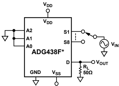
Figure 23. Off Isolation
