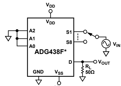
Figure 23. Off Isolation
