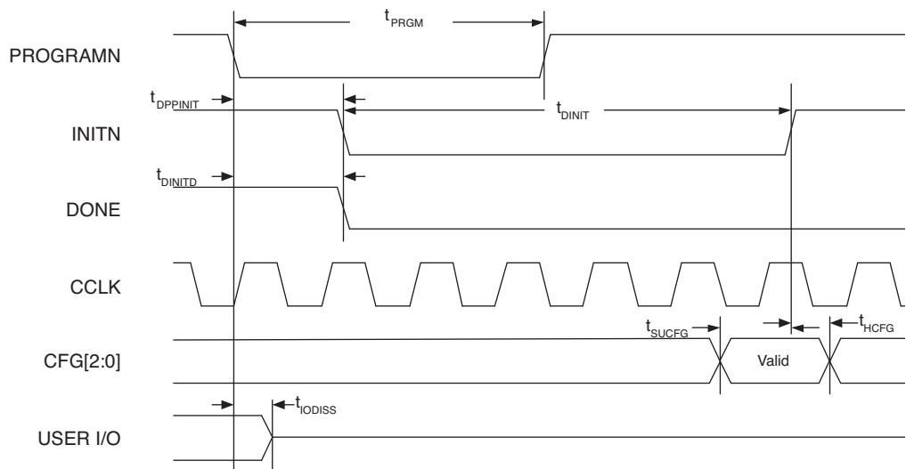
Figure 3-18. Configuration from PROGRAMN Timing
