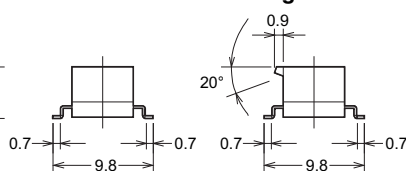
Short actuator
