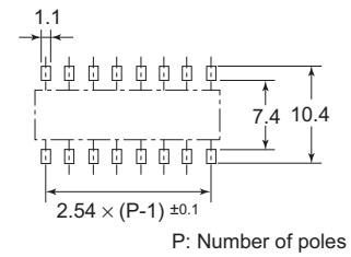
Dimensions of PCB Pad (Reference) (Top View)
