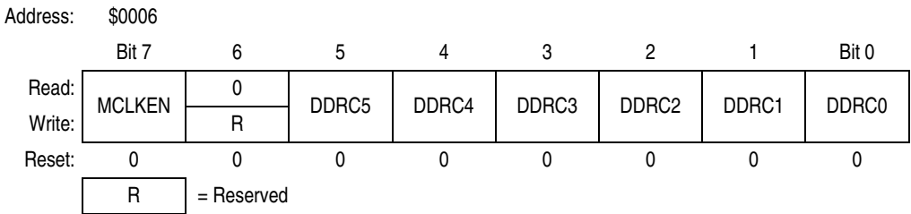
Figure 22-9. Data Direction Register C (DDRC)
