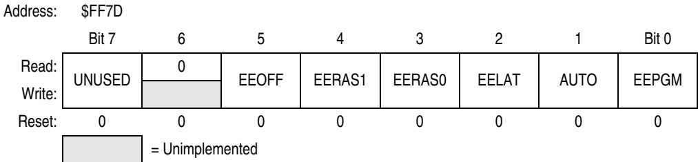
Figure 7-2. EEPROM-2 Control Register (EE2CR)
