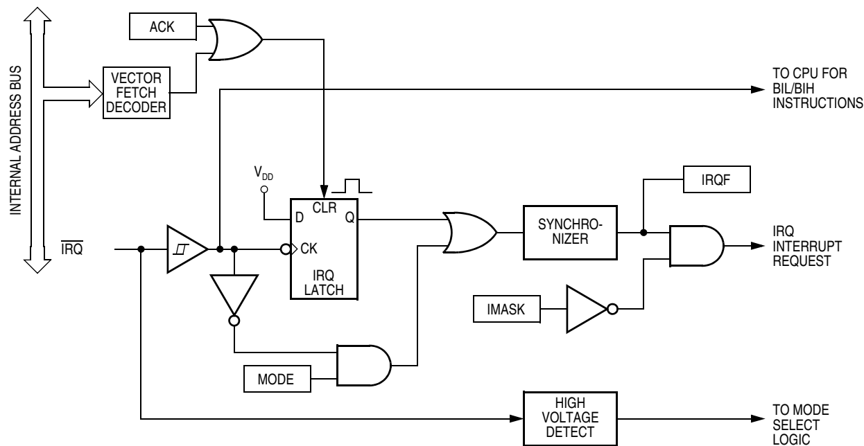
Figure 17-1. IRQ Block Diagram
