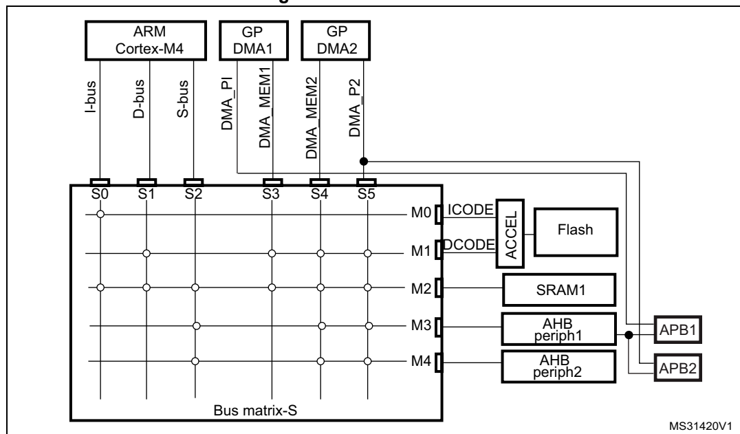
Figure 4. Multi-AHB matrix
