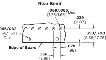
Recommended Mounting Hole Pattern for .062 [1.57] Thick PC Board Using a Right-Angle Header
