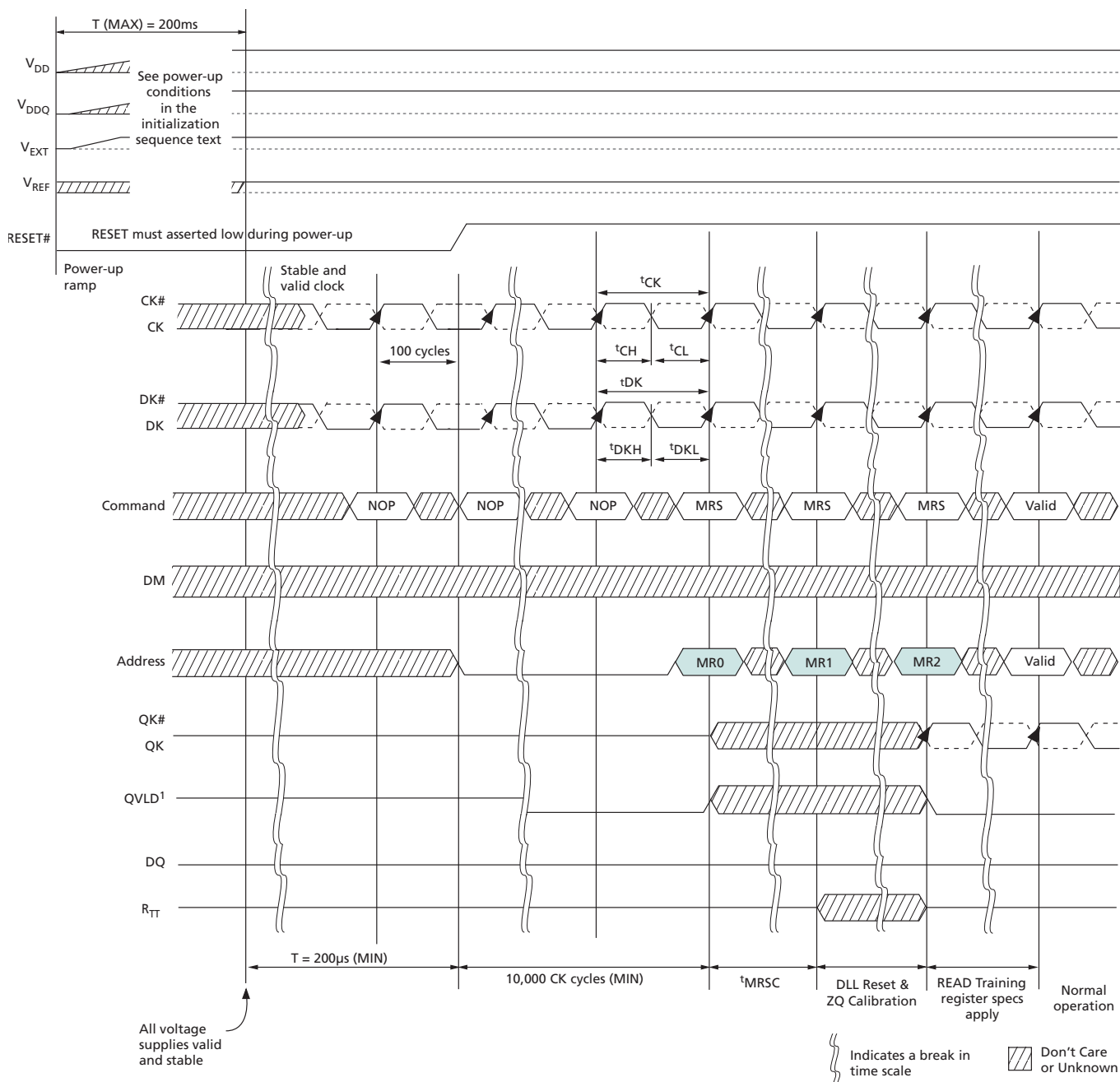
Figure 41: Power-Up/Initialization Sequence
