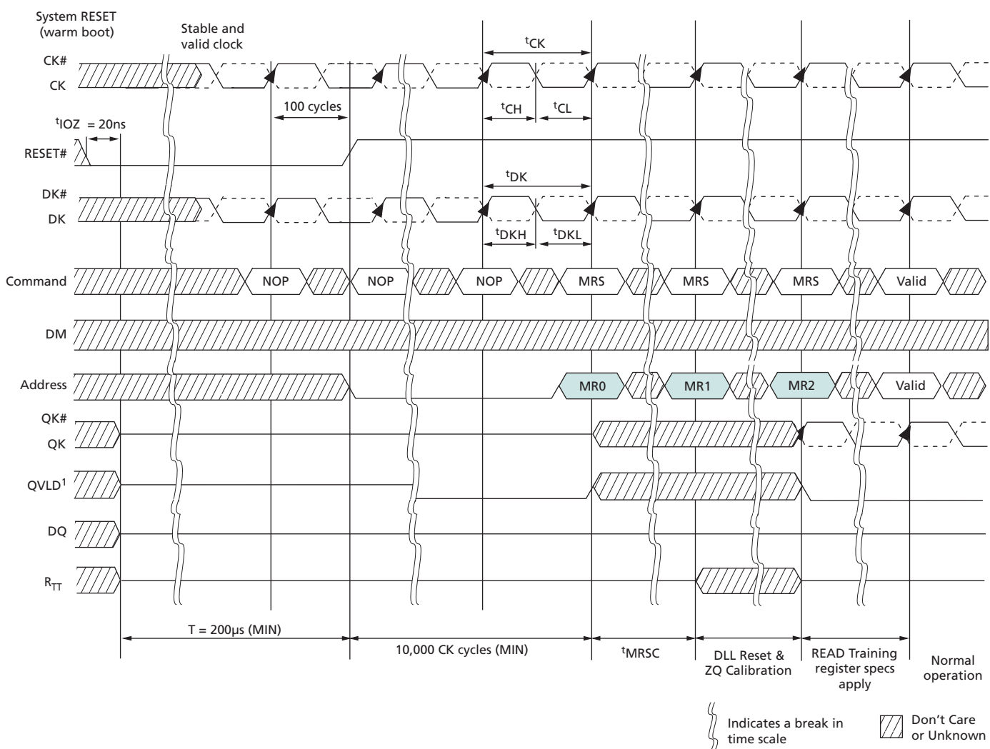
Figure 57: RESET Sequence
