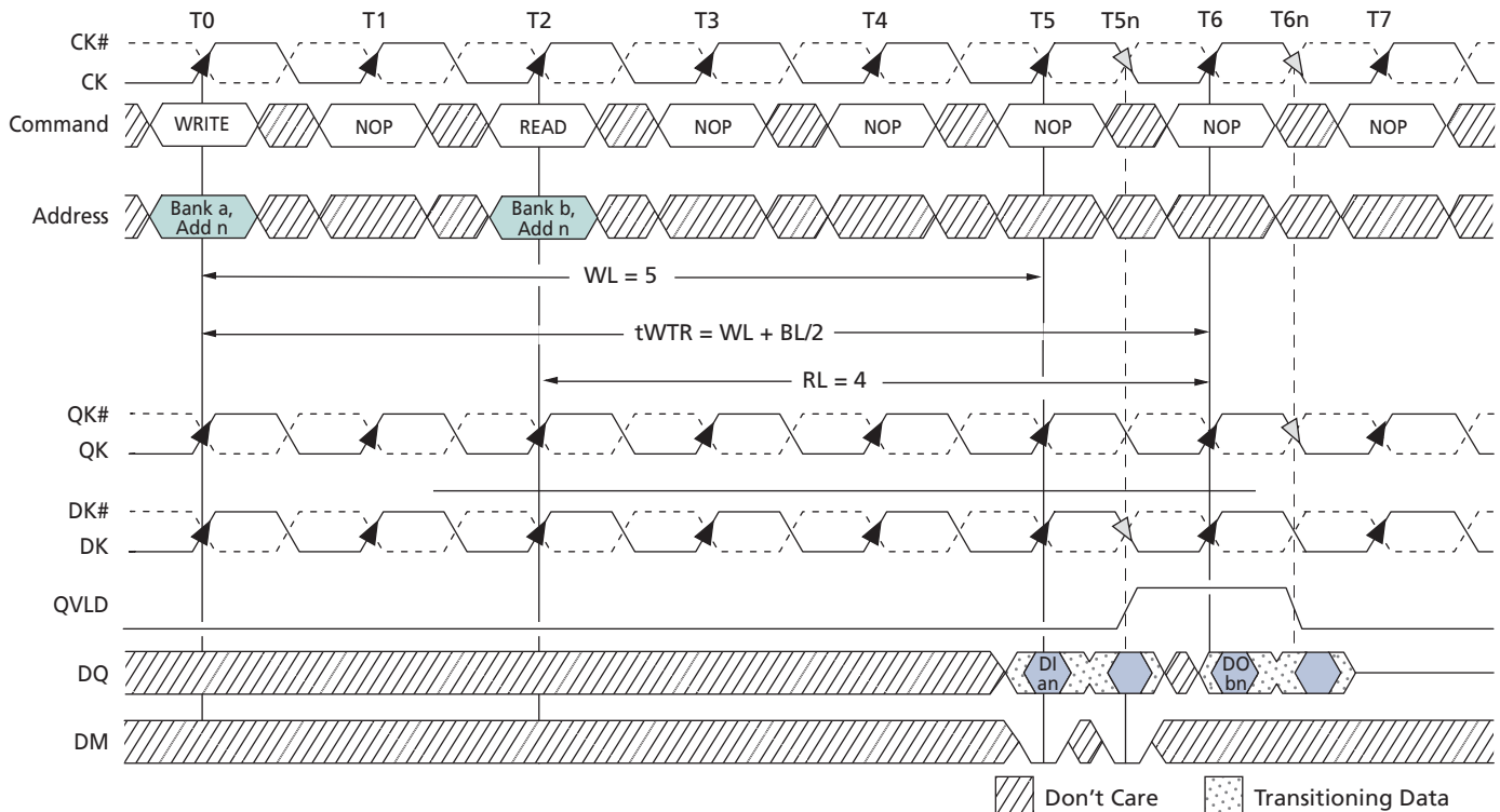
Figure 44: WRITE-to-READ
