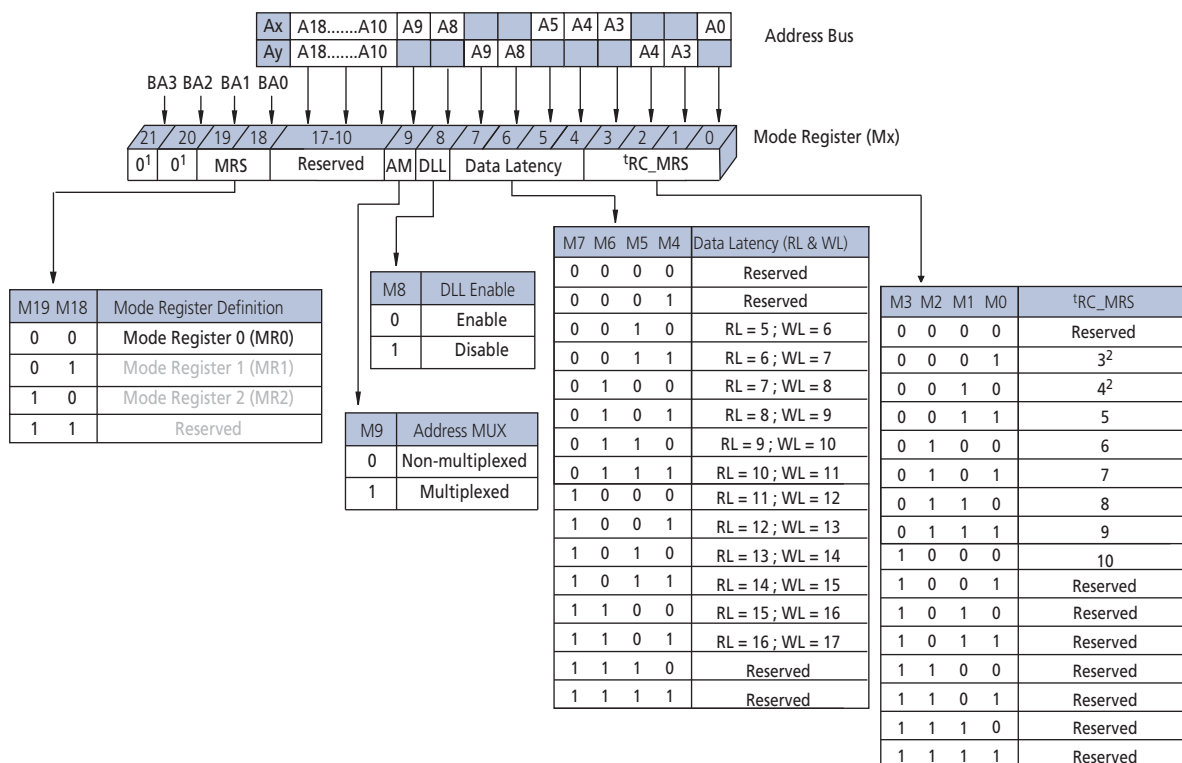
Figure 60: MR0 Definition for Multiplexed Address Mode
