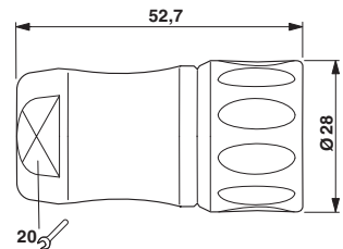
Dimensional drawing
