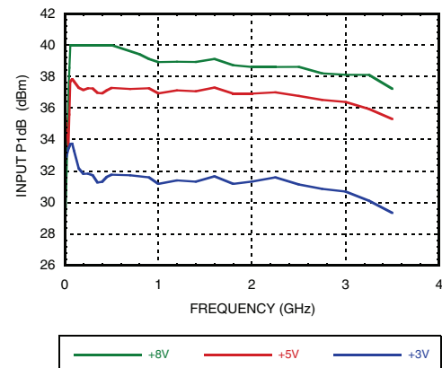
Input P1dB vs. Vctl
