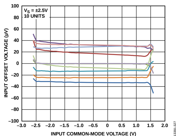
Figure 24. Input Offset Voltage vs. Input Common-Mode Voltage
