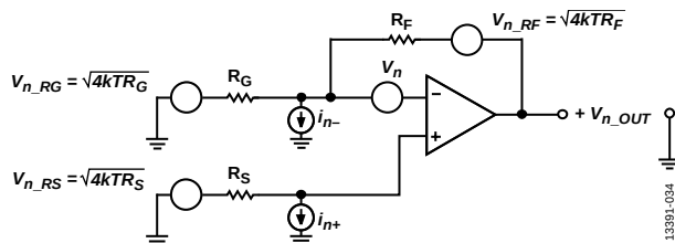
Figure 55. Noise Sources in Typical Connection
