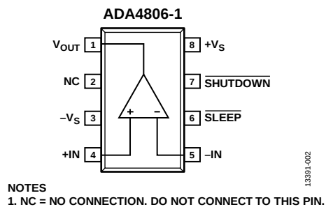
Figure 4. Pin Configuration
