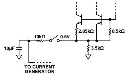
Figure 28. Equivalent VREF Circuit
