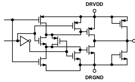
Figure 27. Equivalent Digital Output Circuit
